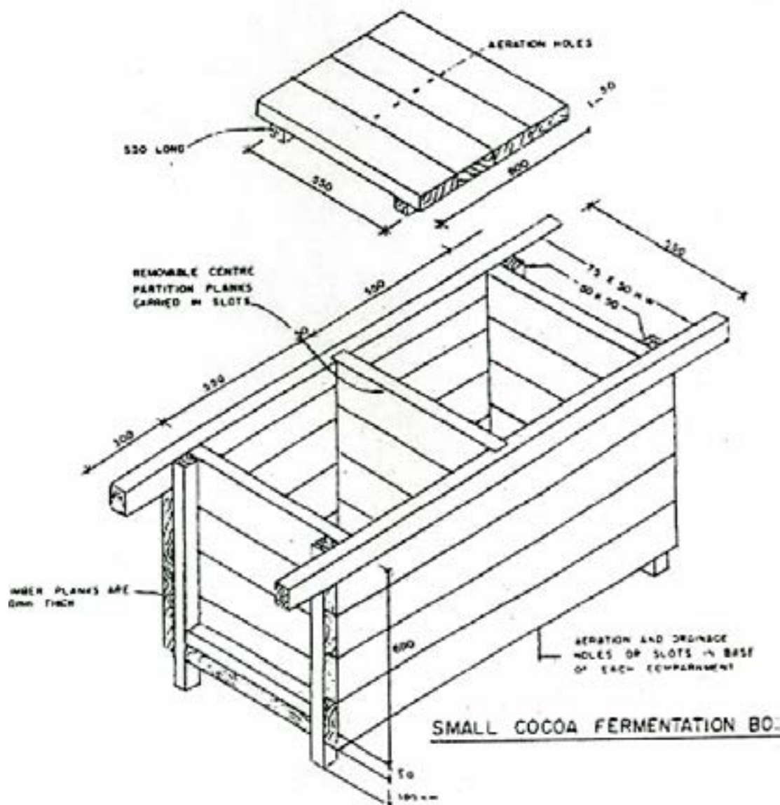
Figure 12.4 Construction plan for a double minibox with a heavy lid – the centre boards can be pulled out of a slot to enlarge the box. Note the handles enabling the box to be carried. Box is 1100mm long x 550mm wide x 600mm deep, constructed of planks 50mm thick, with gaps left between bottom planks for drainage
