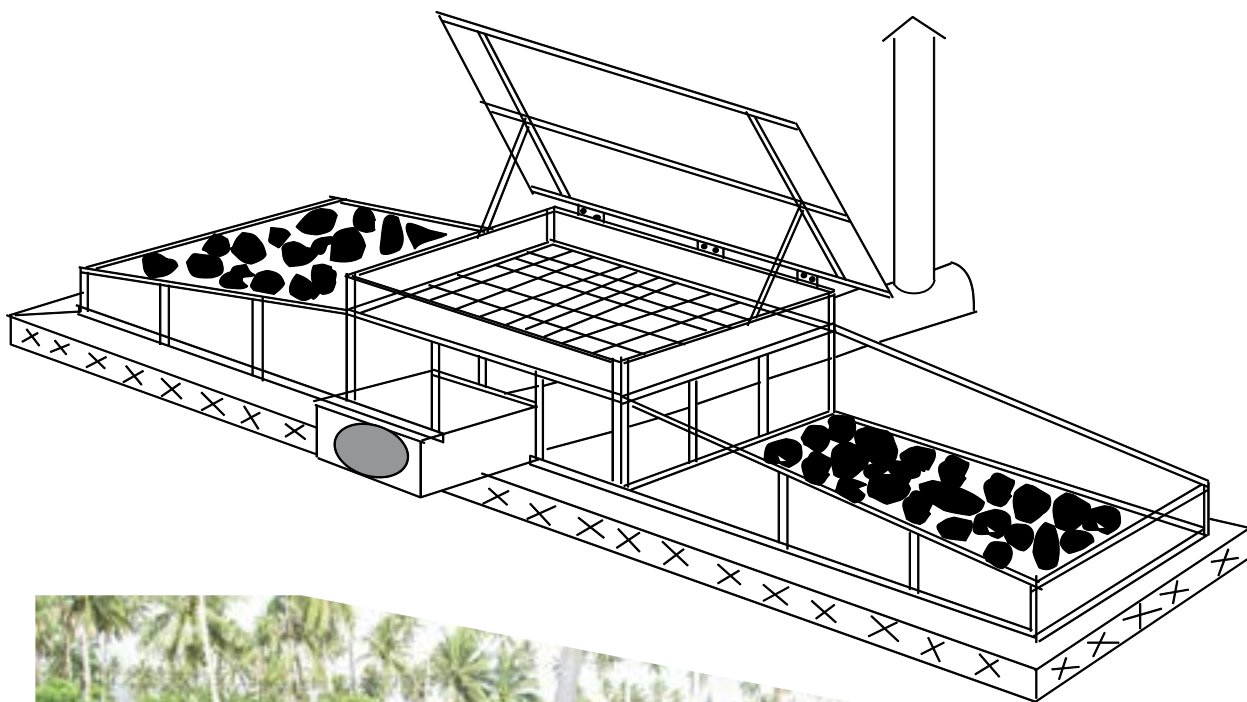
Figure 12.16 – Plan drawing of a combined solar/wood-fired kiln drier developed at CCIL – black painted rocks on the sides are heated by the sun and air flowing over them and through the rack dries the cocoa; during rain the standard wood-fired kiln can be used to continue drying of the beans
